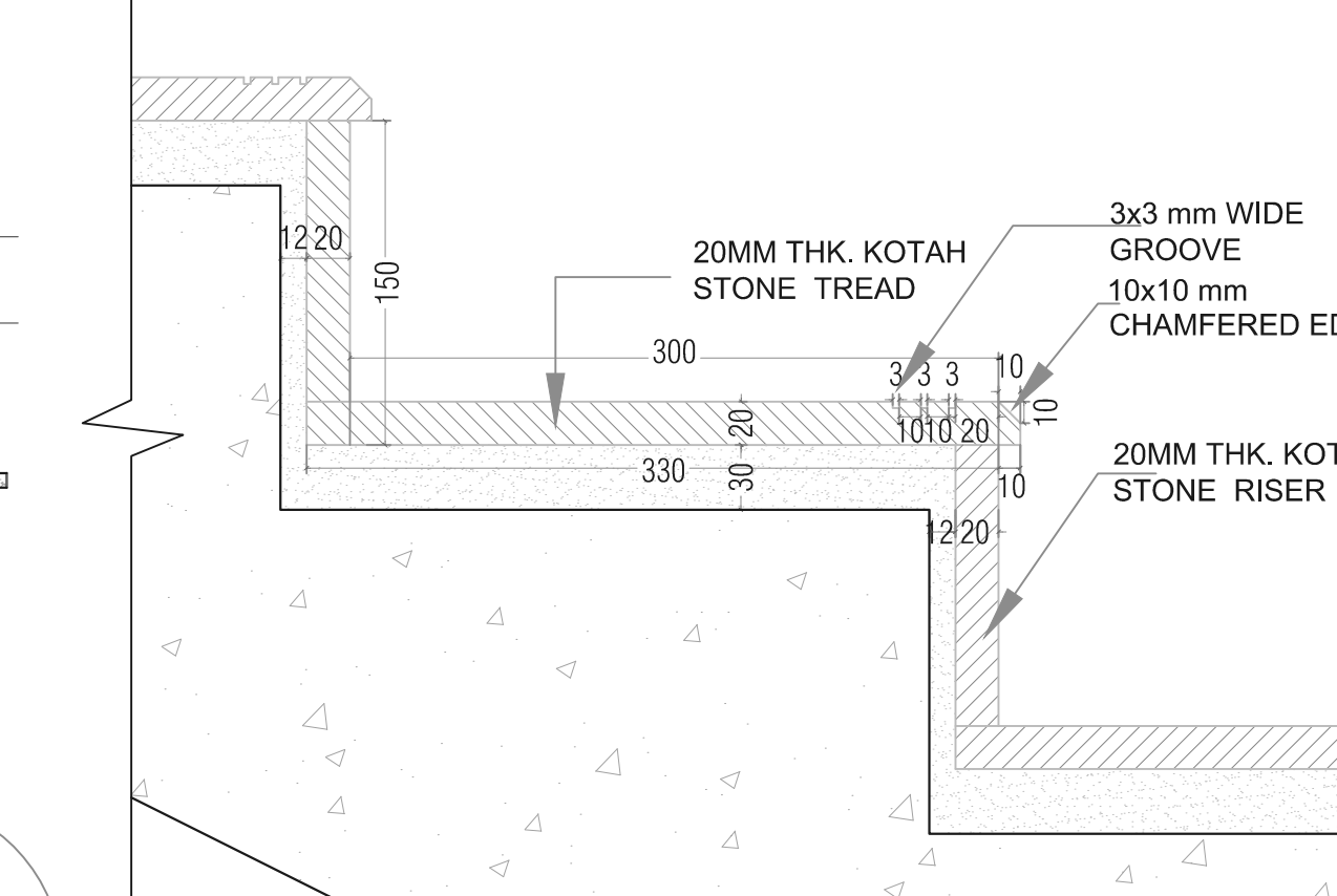
2 DETAIL 1:5
